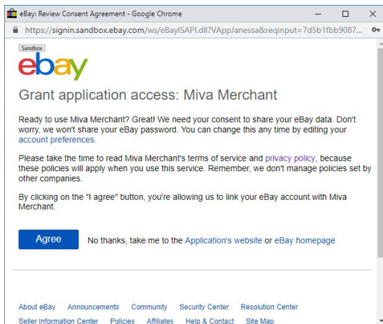
Figure 3: Consent Agreement
